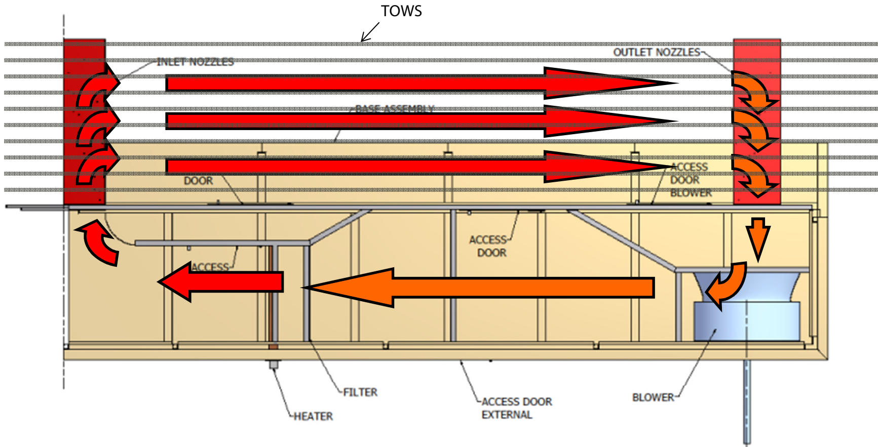
TOP VIEW
