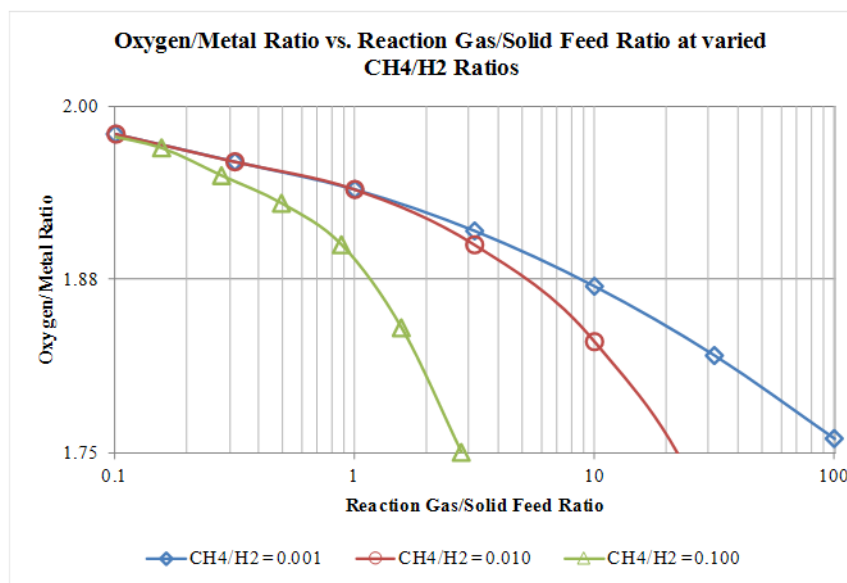
Figure 5. The target reaction completion was a reduction in the ratio of oxygen/metal atoms in the product from 2 to 1.75.
